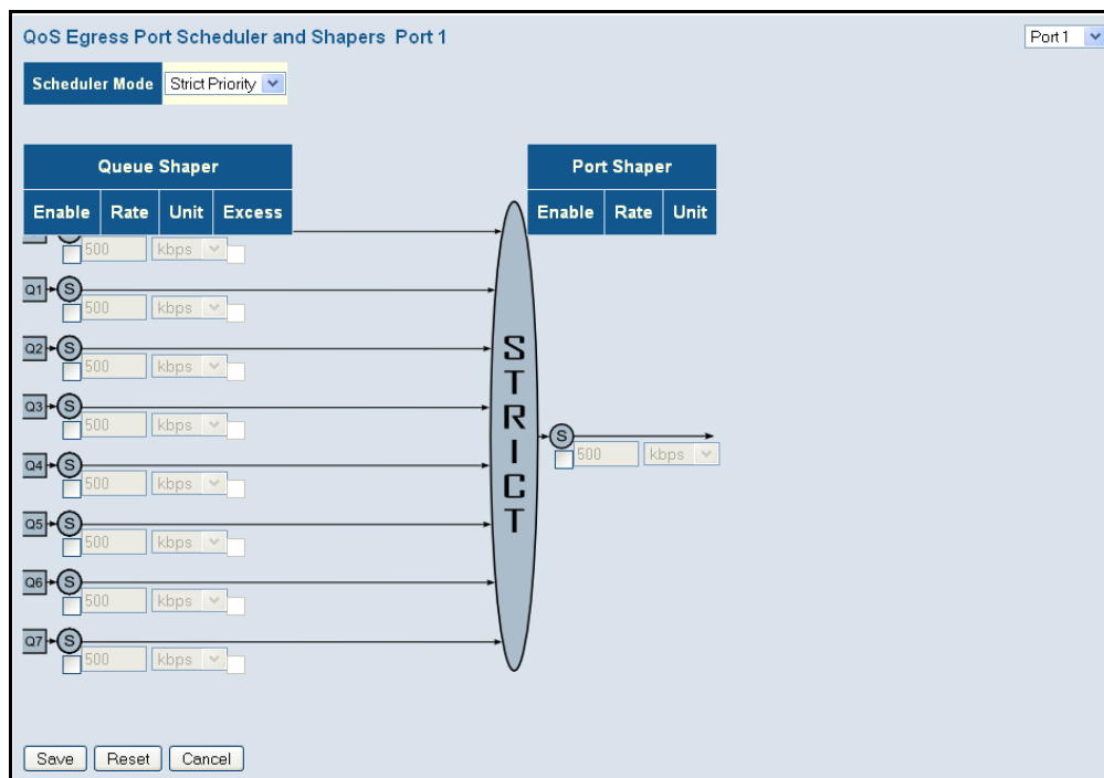
Figure 73: Configuring Egress Port Schedulers and Shapers
