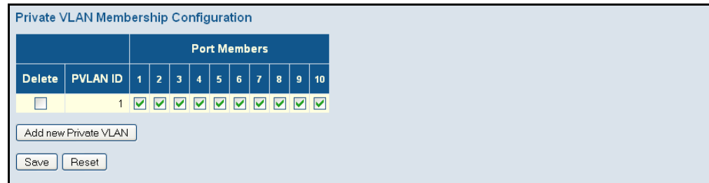
Figure 63: Private VLAN Membership Configuration
