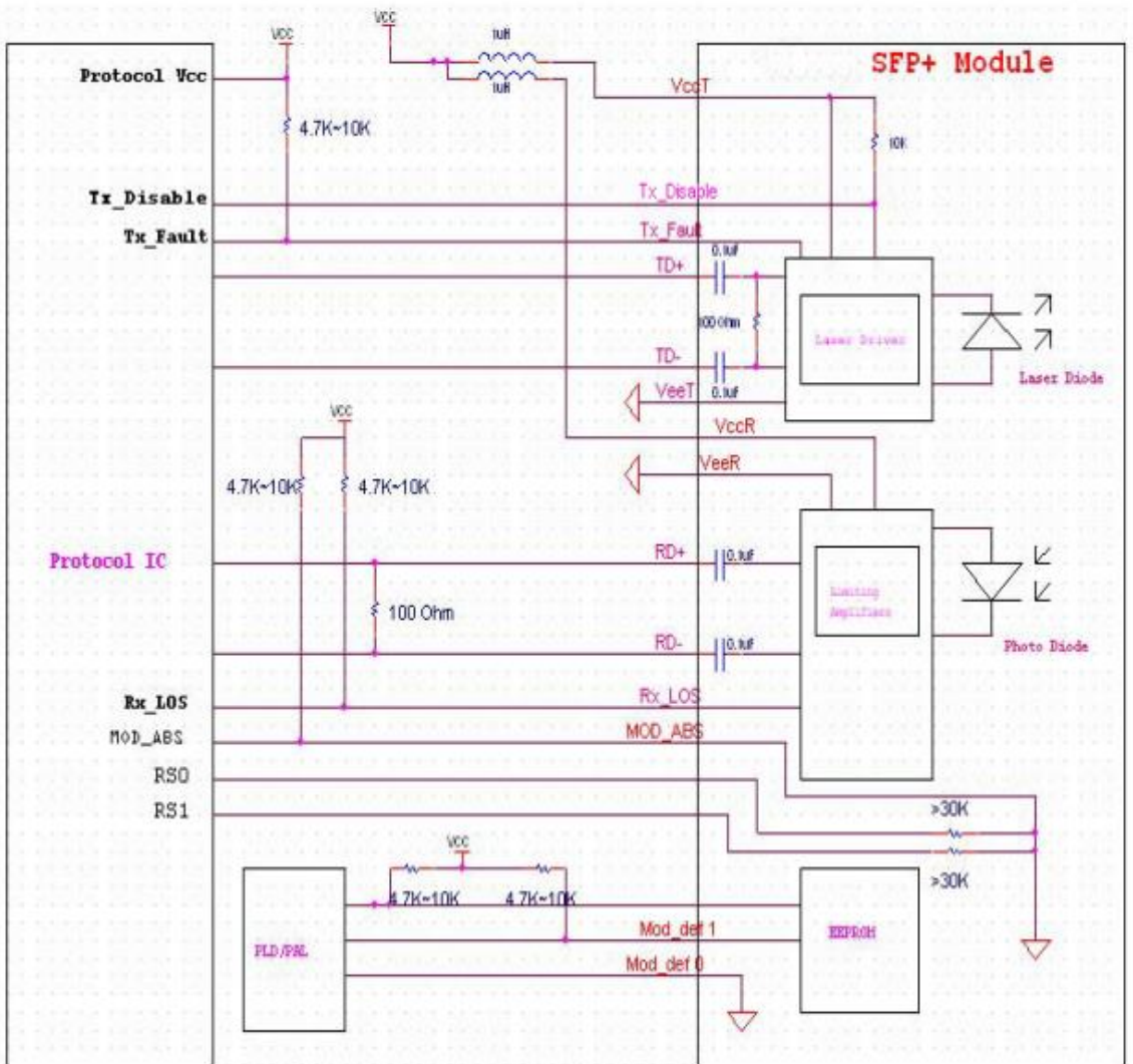
Figure4. Host-Module Interface
