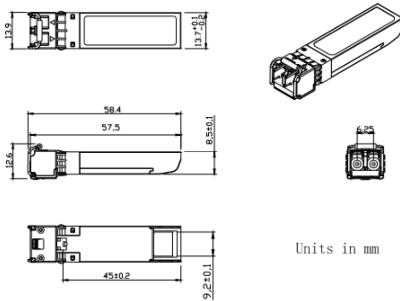
Figure5. Mechanical Specifications
