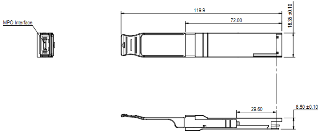
Figure 5. Mechanical Outline
