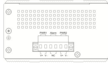
Figure 4. Terminal Block
