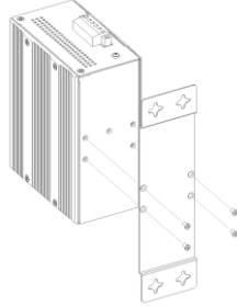
Figure 8. Wall Mount
