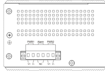
Figure 4. Terminal Block
