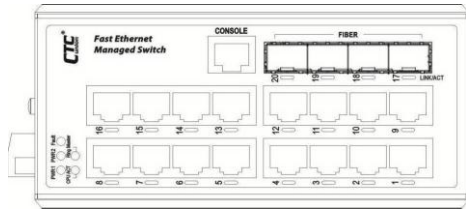
Figure 1. Front Panel
