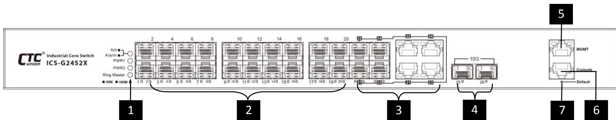
Figure 2. ICS-G24S2X Front Panel
