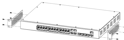
Figure 13. Attaching Rack-Mounting Brackets
