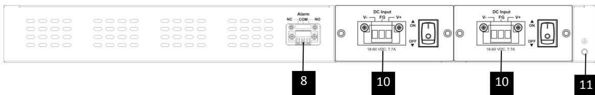
Figure 5. Rear Panel with 2 DC Power Supplies
