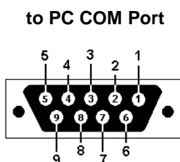
Figure 7. RS232 (Female) Pinouts
