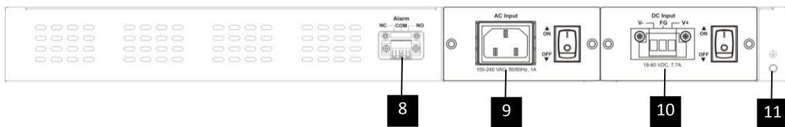
Figure 3. Rear Panel with 1 AC and 1 DC Power Supply
