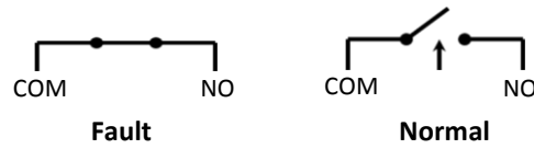
Figure 12. Alarm Relay for NO (Normally Open) Type
