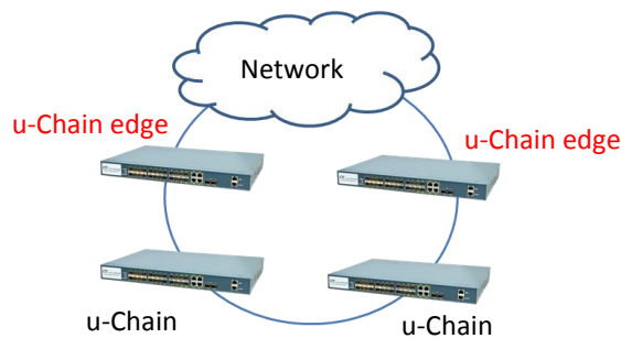
Figure 3. u-Chain ring connects to a network
