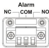
Figure 10. Alarm Relay Terminal Block
