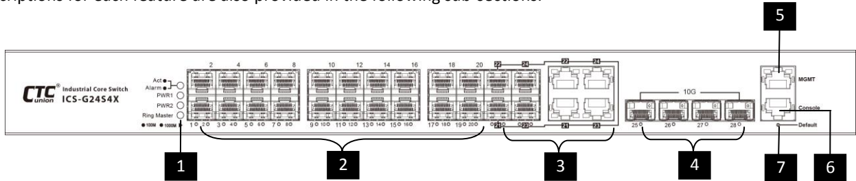
Figure 1. ICS-G24S4X Front Panel
