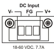
Figure 9. Terminal Block (DC) Power Connector Pin Assignment
