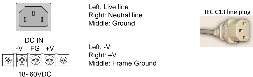
Figure 4. IEC (AC) & Terminal Block (DC) Power Connector Pin Assignment
