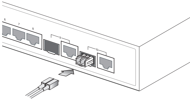
Figure 4-3 Making Fiber Port Connections
