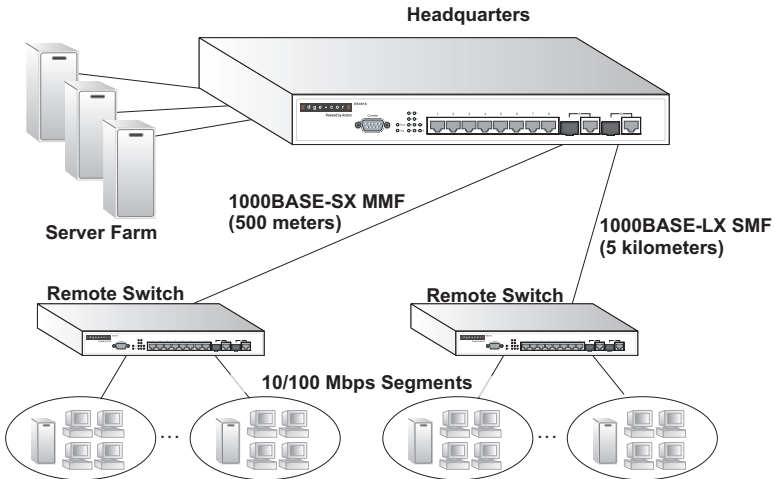
Figure 2-3 Remote Connections with Fiber Cable
