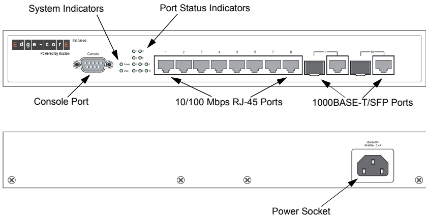
Figure 1-1 Front and Rear Panels
