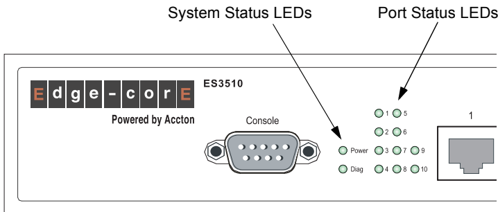
Figure 1-2 Port LEDs
