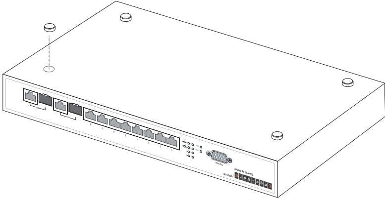
Figure 3-4 Attaching the Adhesive Feet
