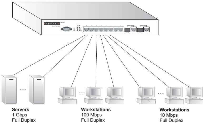
Figure 2-1 Collapsed Backbone
