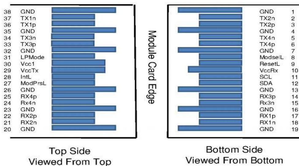
Figure1 Top Side and Bottom Side of QSF28
