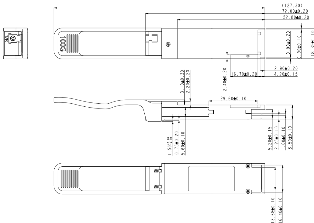
Figure3 100G ER1 BiDi QSFP28 Mechanical Dimensions
