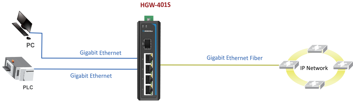
HGW-401S Gigabit Ethernet Switch Application
