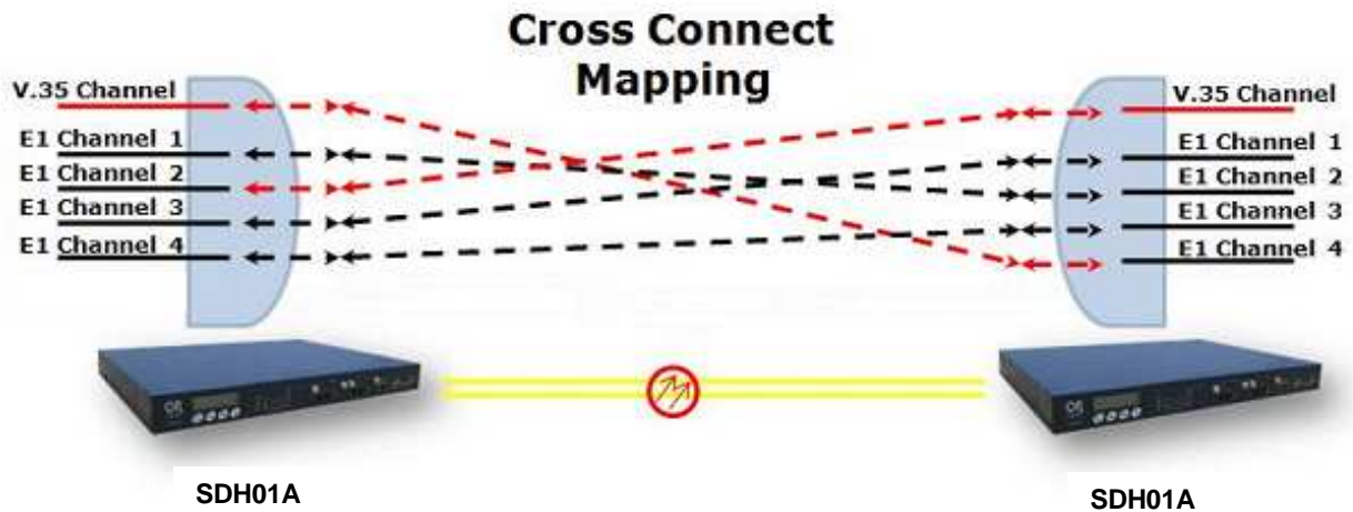
Figure 2-4 Cross Connect Mapping
