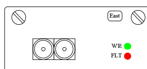
Figure 3-5 Optical interface LED Indicators
