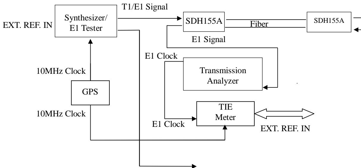
Figure 6-1 The frequency tractability connected
