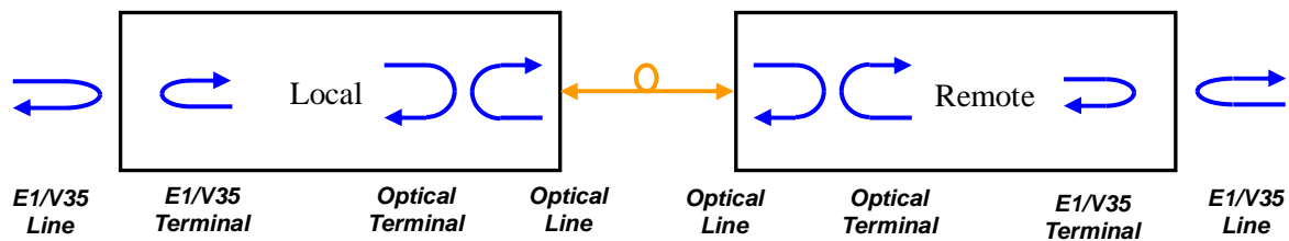
Figure 6-2 Loopback definitions
