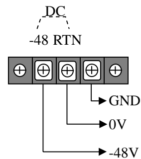
Figure 3-8 DC Modules Connection
