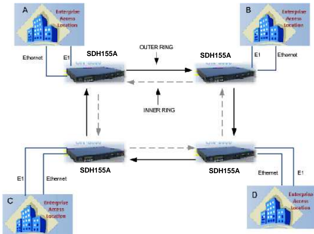
Figure 2-5 EoS (Ethernet over SDH) ring protection scheme
