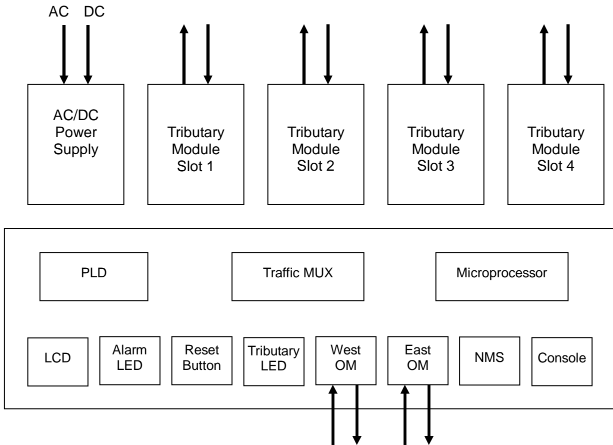
Figure 1-2 SDH01A Block diagram
