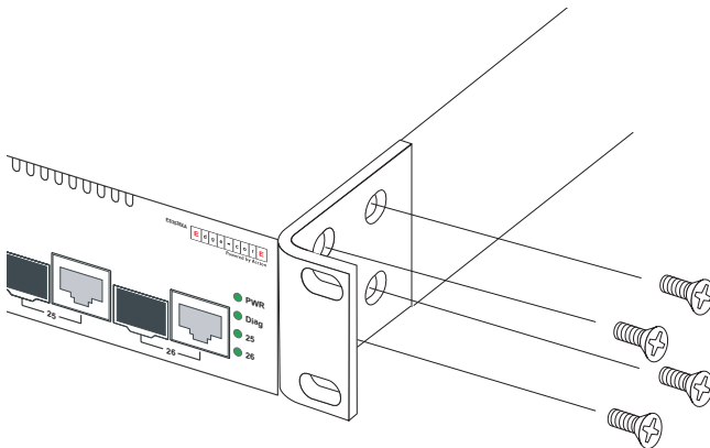
Figure 3-2 Attaching the Brackets
