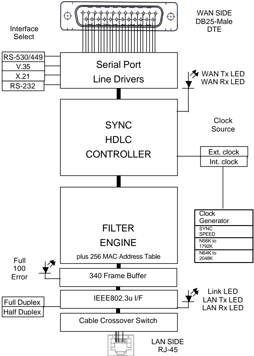
Figure 1: ET100 Functional Block Diagram
