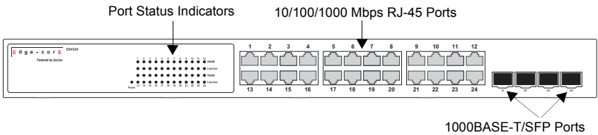
Figure 1-1 Front Panels
